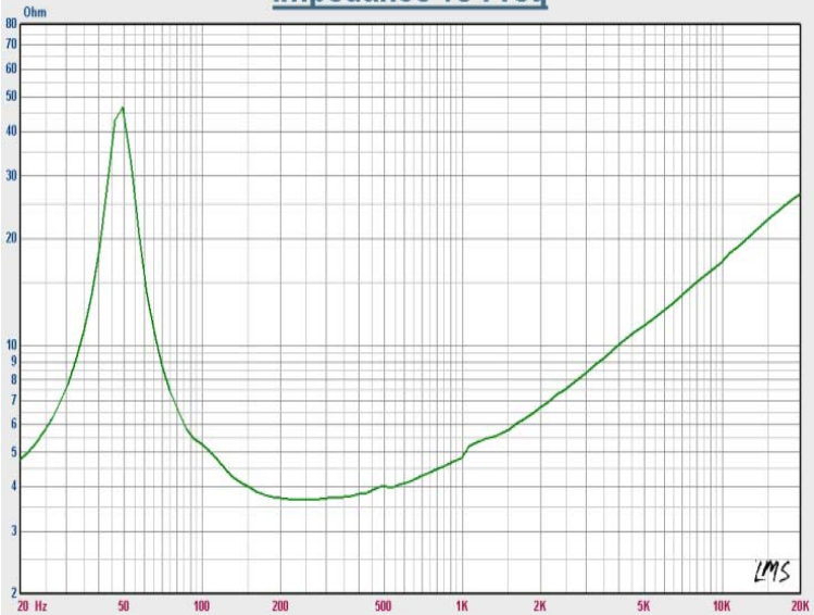
Impedance vs Freq
